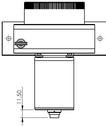
C connection connector M16 8 pins DIN
